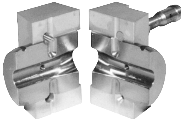
Steel Stripper Jaws with O-Ring Detection.
